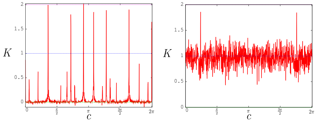
Figure 5: Dependence of the asymptotic growth rate K on the frequency c . (a) regular dynamics at 0.9\text{Hz} and (b) chaotic dynamics at 0.6\text{Hz} .
