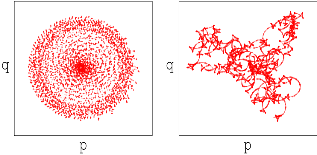
Figure 3: The dynamics of the translation components (p, q) of the E(2) extension. (a) bounded trajectories are shown corresponding to periodic dynamics at \omega = 0.9 \text{Hz} . (b) Brownian-like trajectories are shown corresponding to chaotic dynamics at \omega = 0.6 \text{Hz} . Both cases show 2700 data points and are calculated for c = 1.95 .
