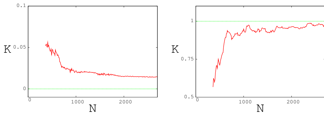
Figure 6: Dependence of the asymptotic growth rate K on the length of the time series N . (a) periodic case \omega = 0.9\text{Hz} . (b) chaotic case \omega = 0.6\text{Hz} . We used the data set corresponding to the full 9 minutes of recording, taking every 5th data point, so the maximum value of N is 2700.
