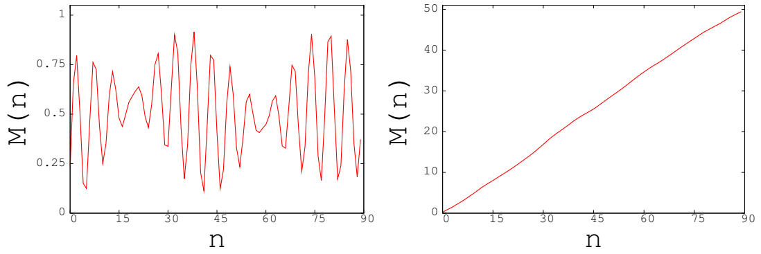
Figure 4: Mean square displacement M(n) as a function of n for 900 data points shown from n = 0 up to n = 90 . (a) periodic case \omega = 0.9\text{Hz} corresponding to Fig. 3a. (b) chaotic case \omega = 0.6\text{Hz} corresponding to Fig. 3b. Both cases are calculated for c = 1.95 .
