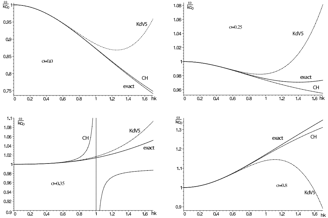
Figure 1: Normalised dispersion relations for \sigma = 0.0, 0.25, 0.35, 0.8 as a function of hk . The full line is the exact phase speed (44); the dashed line is the approximation (43) and the short dashed line is that of KdV5.
